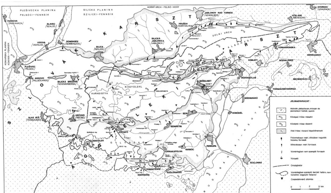
Figure 49 : The Aggtelek Karst (Maucha et al. 2000)
