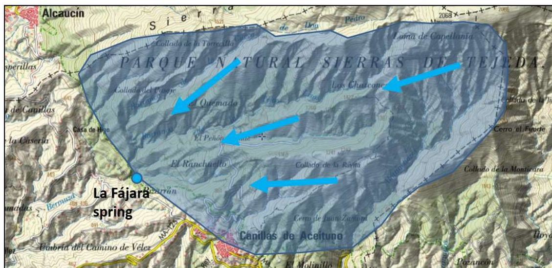
Figure 53: Directions of the flow of groundwater in the catchment area "La Fajara"
