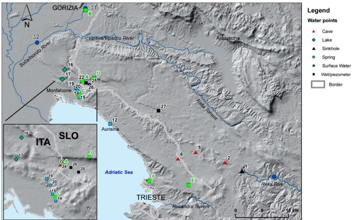
Figure 34: Digital elevation model of the Classical Karst area (Calligaris et al., 2018)
